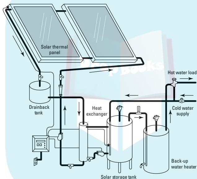
Figure 12-4: A drainback- style, solar water heater system.
